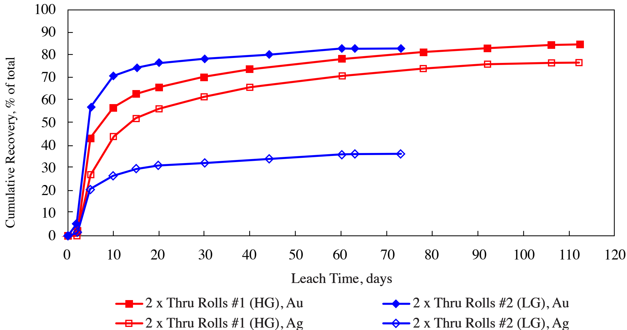
Figure . - Gold and Silver Leach Rate Profiles, Colum Leach Tests, Moss Project, 2 x Thru Rolls #1 (HG) and 2 x Thru Rolls #2 (LG), P 95 1/4" Feeds
